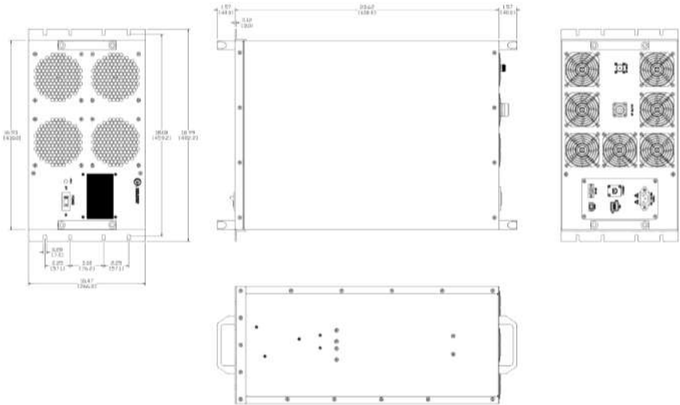
OUTLINE DRAWING SHOWN WITH LCD DIGITAL CONTROLLER
